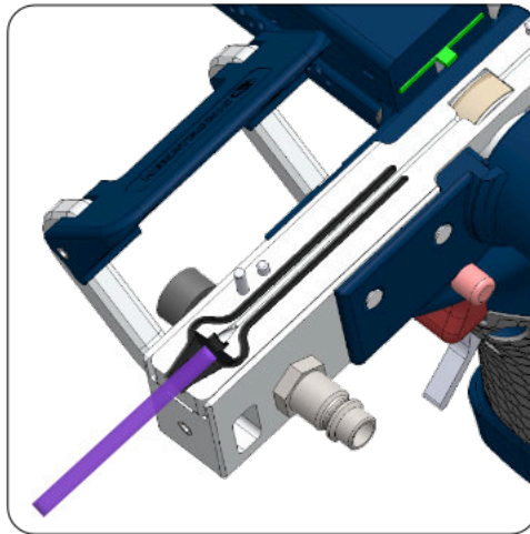
10. Open the clamp, lift the top body and place the duct onto the nozzle, hold whilst closing the clamp. (for pre-connectorized fibre: push the ferrul into the duct before closing the lever).
