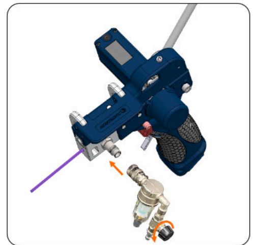
11. Connect the air filter and valve assembly to the tool - open the valve - turn anticlockwise.
