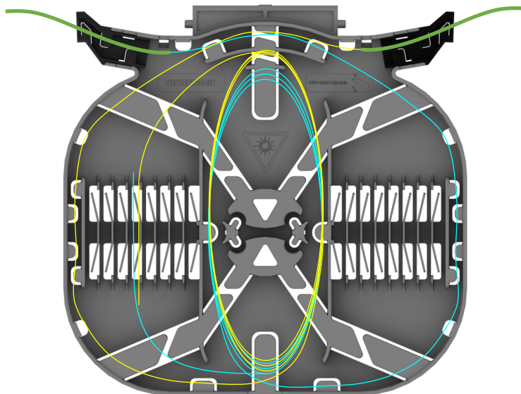
Left hand splice routing
