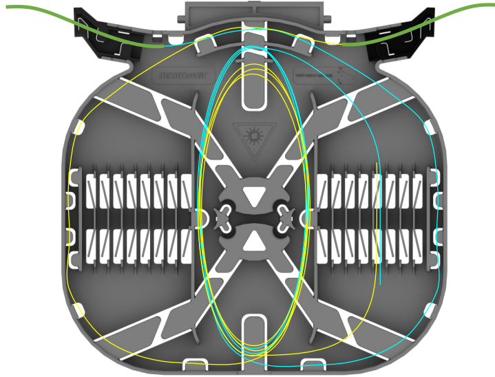
Right hand splice routing
